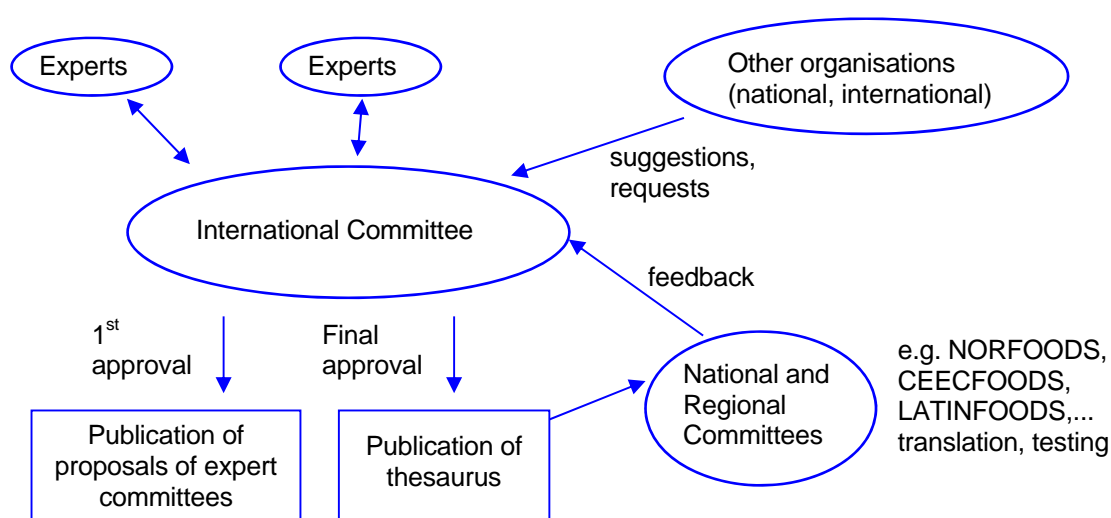
Figure 1. information flow
